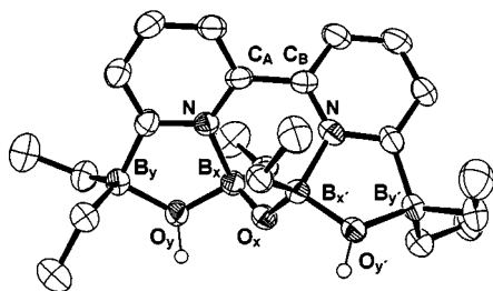
Figure 3. Structure of 5 in the crystal; selected bond lengths [Å] [mean values and range given (esd. 0.006–0.009 Å)]: B X –O X 1.440 (1.415–1.445), B X –O Y 1.525 (1.503–1.536), B Y –O Y 1.595 (1.561–1.620), B X –N 1.626 (1.611–1.650), C A –C B 1.486 (1.479–1.494)
