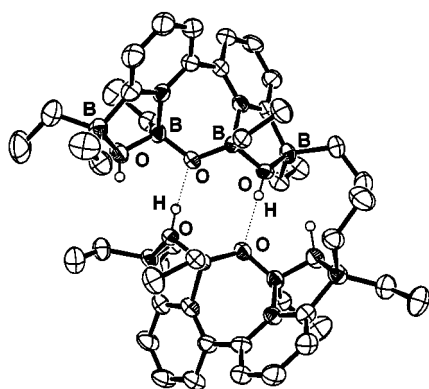
Figure 4. Hydrogen-bridged dimer of 5 in the crystal
