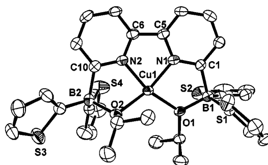
Figure 2. Structure of 4 in the crystal; selected bond lengths [Å] and angles [°]: B1–C1 1.630(6), B1–O1 1.558(5), B2–O2 1.575(5), Cu1–N1 1.938(3), Cu1–N2 1.938(3), Cu1–O1 1.962(3), Cu1–O2 2.016(3), C5–C6 1.483(6), C1–B1–O1 103.7(3), C10–B2–O2 104.8(3), N1–Cu1–N2 80.8(1), N1–Cu1–O1 83.1(1), O1–Cu1–O2 114.8(1), O2–Cu1–N2 83.4(1), B1–O1–C27 116.6(3), C27–O1–Cu1 126.5(3), Cu1–O1–B1 116.9(2), N1–C5–C6–N2 7.4, N1–C1–B1–O1 2.1, N2–C10–B2–O2 23.7
