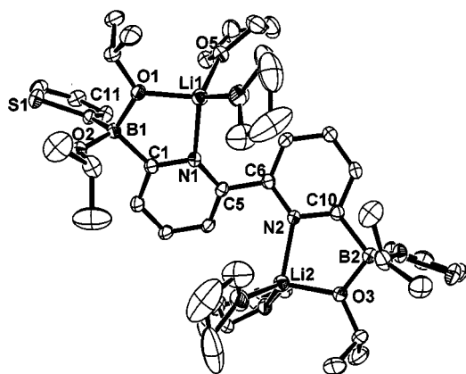
Figure 1. Structure of 2f in the crystal; selected bond lengths [Å] and angles [°]: B1–C1 1.642(8), B1–O1 1.506(7), B1–O2 1.479(7), Li1–O1 1.87(1), Li1–N1 2.08(1), Li1–O5 1.97(1), C1–B1–O1 106.4(4), C1–B1–O2 112.5(5), C1–B1–C11 107.0(4), N1–C5–C6–N2 30.6
